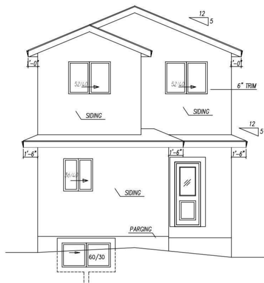
REAR ELEVATION
